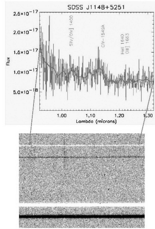
Figure 2: Bi-dimensional spectrum of the most distant QSO, at the time, at z=6.41 in the bottom panel. The extracted spectrum is shown in the upper panel. A fit to the spectrum is also shown, where several broad emission lines are identified. The most intense feature is the CIV line, detected with a S/N ratio of 10. The spectrum is the co-addition of 5 frames of 850 s exposure time each, giving an approximate total time of 70 minutes.
